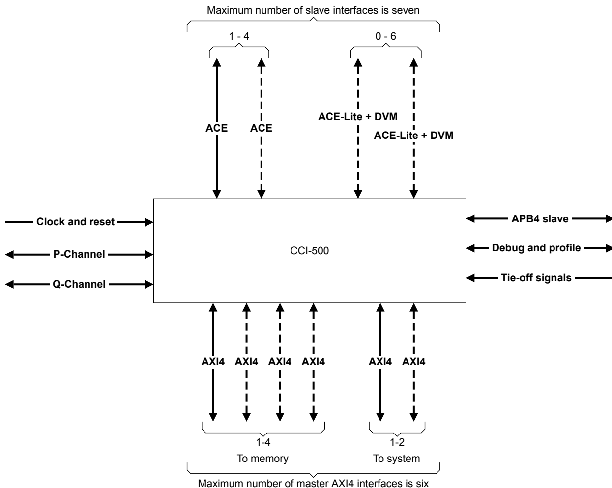
Figure 2-1 CCI-500 interfaces
