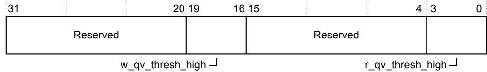
Figure 3-5 qos_threshold register bit assignments
