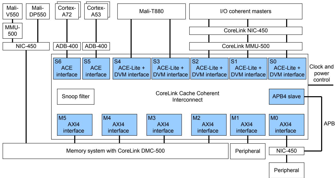
Figure 1-1 Example system with a CCI-500
