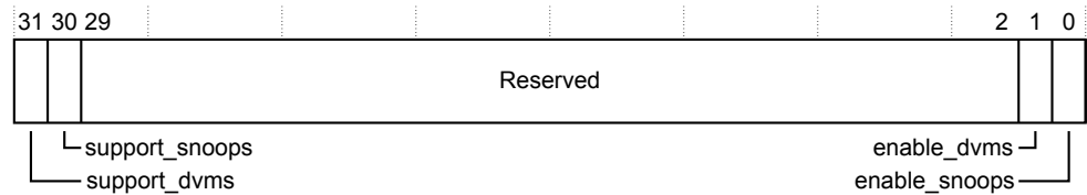
Figure 3-8 snoop_ctrl register bit assignments
