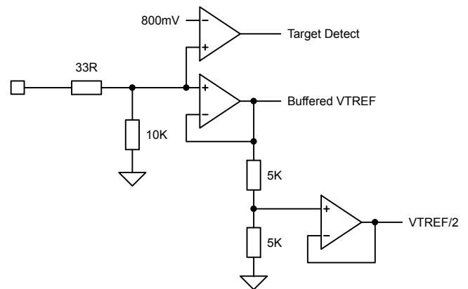
Figure 1-16 VTREF signals
