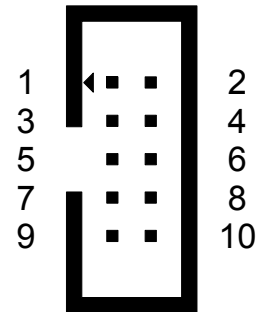
Figure 2-8 User I/O connector pinout
