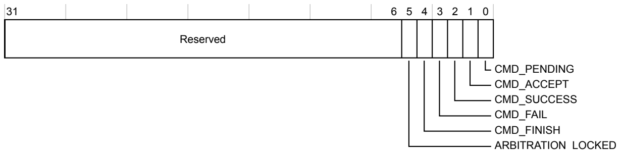
Figure 3-12 STATUS register bit assignments
