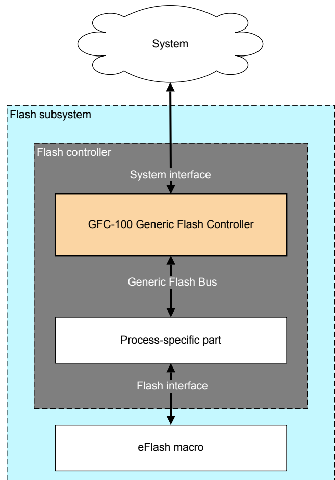
Figure 1-1 GFC-100 in a Flash controller implementation
