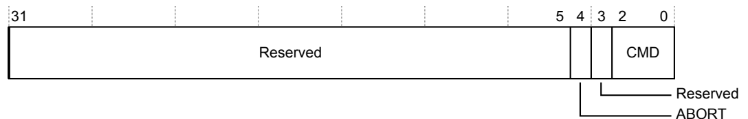
Figure 3-11 CTRL register bit assignments
