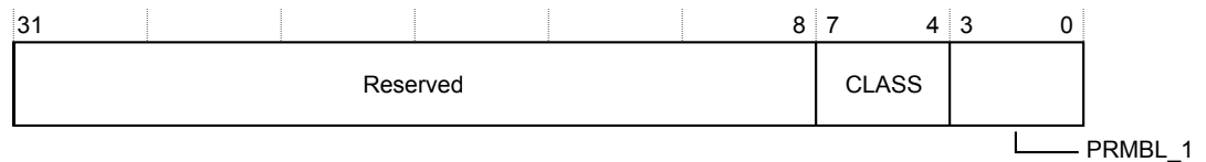
Figure 3-24 CIDR1 register bit assignments
