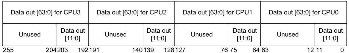
Figure 2-10 MBISTOUTDATA[255:0] format for Outer RAM
