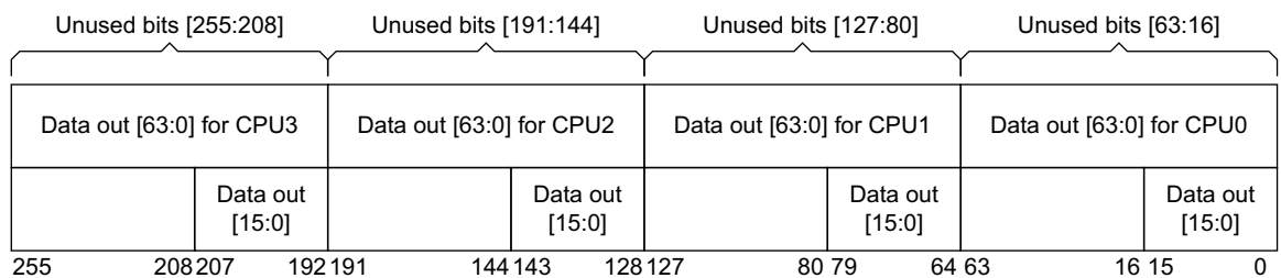
Figure 2-16 MBISTOUTDATA[255:0] format for GHB RAM in normal mode
