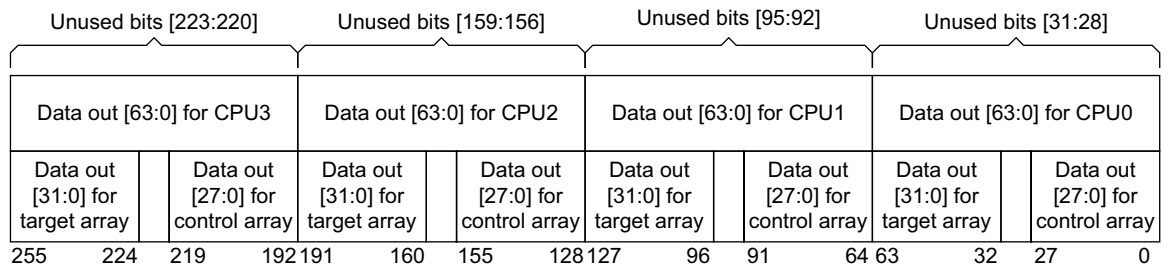
Figure 2-12 MBISTOUTDATA[255:0] format for BTAC RAM
