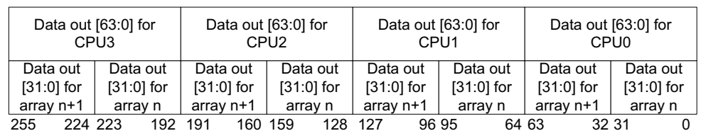
Figure 2-2 MBISTOUTDATA[255:0] format for Instruction data RAM and Data data RAM
