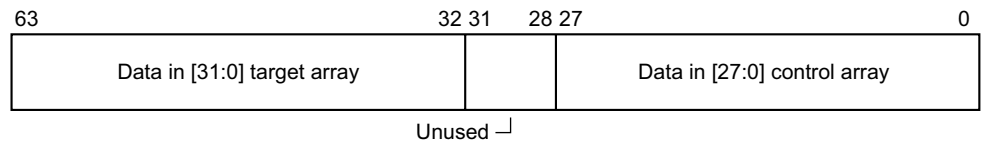
Figure 2-11 MBISTINDATA[63:0] format for BTAC RAM
