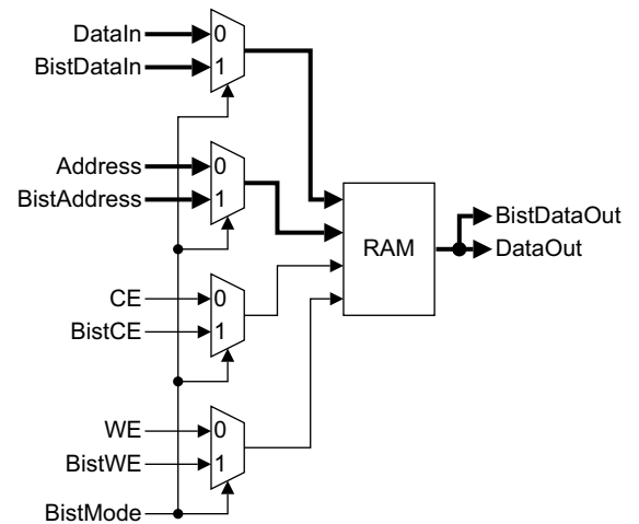
Figure 1-4 Traditional method of interfacing MBIST
