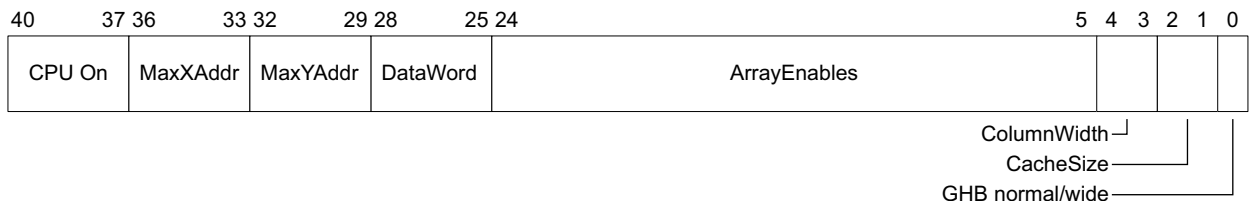
Figure 3-2 MBIST instruction register dispatch unit
