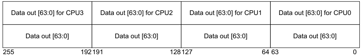
Figure 2-18 MBISTOUTDATA[255:0] format for GHB RAM in wide mode
