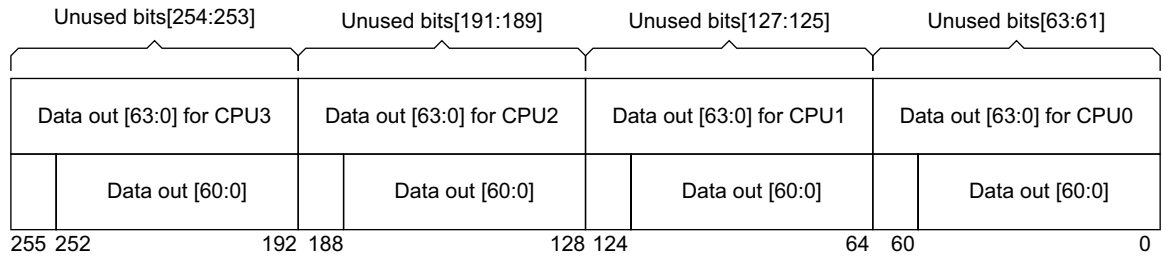
Figure 2-14 MBISTOUTDATA[255:0] format for TLB RAM
