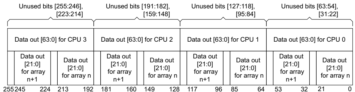
Figure 2-4 MBISTOUTDATA[255:0] format for Instruction tag RAM
