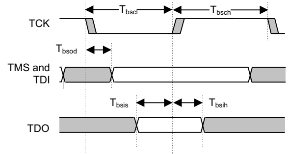
Figure 3-1 JTAG port timing diagram
